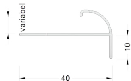
Treppenkantenprofil 40x10x6mm variabel ASM G, L=300cm
